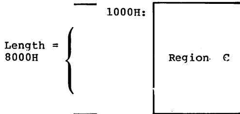
Figure 4-2. Example Memory Region
