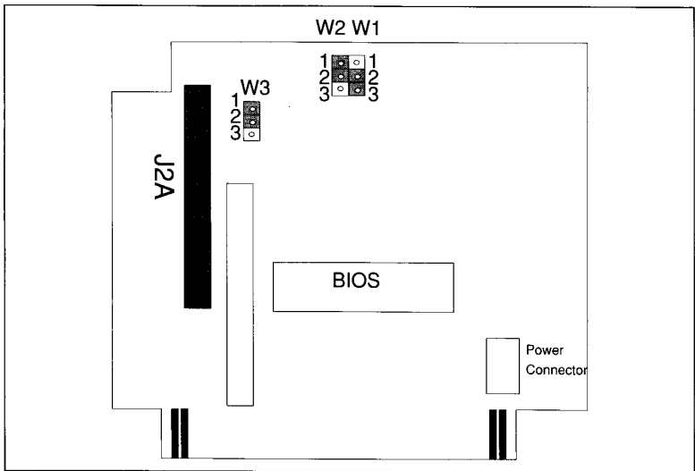
Figure 1-1. WDXT-150 Jumper Locations
