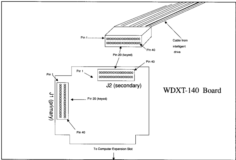
Figure 1-2. Connect Pin 1 to Pin 1
