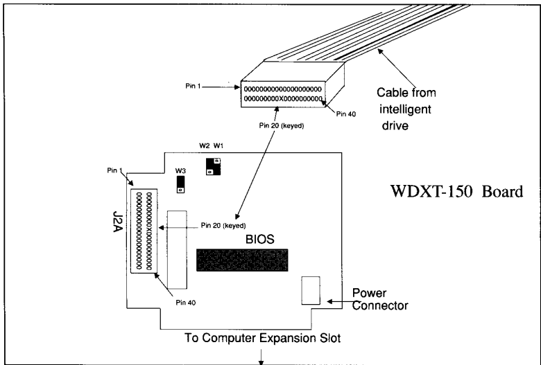
Figure 1-3. Connect Pin 1 to Pin 1
