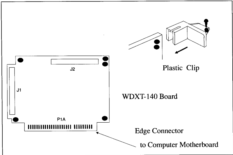
Figure 1-4. Installing Clip
