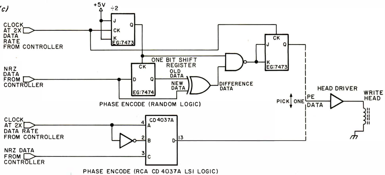
PHASE ENCODE (RCA CD 4037A LSI LOGIC)
